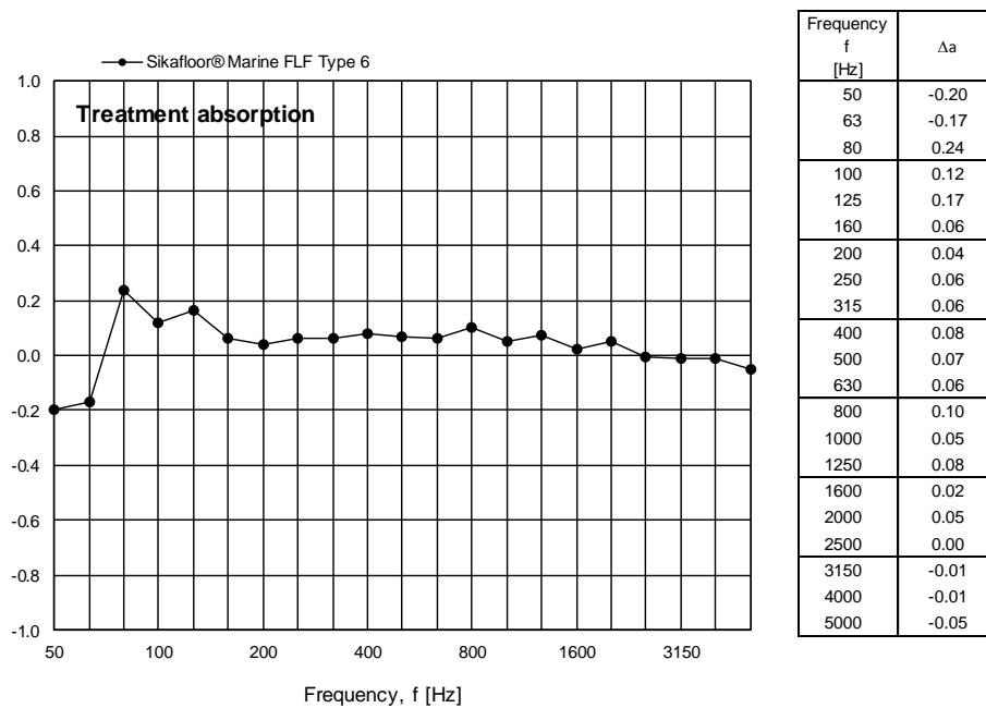
Figure 16 Measured treatment absorption for Sikafloor® Marine FLF Type 6 per one-third octave frequency band.
