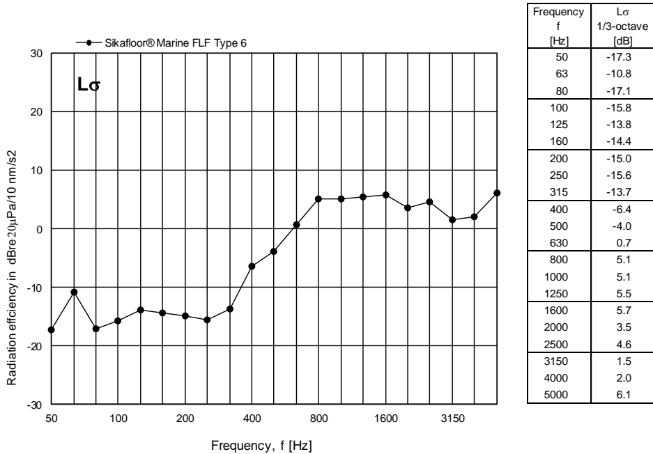
Figure 12 Measured radiation index L_{\sigma} for Sikafloor® Marine FLF Type 6 expressed in dB per one-third octave frequency band.
