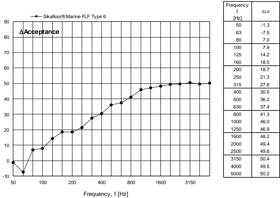
Figure 14 Measured change in acceptance for Sikafloor® Marine FLF Type 6 expressed in dB per one-third octave frequency band.
