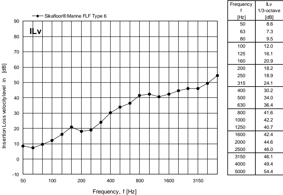
Figure 6 Measured insertion loss IL_v for Sikafloor® Marine FLF Type 6 expressed in dB per one-third octave frequency band. The insertion loss IL_v refers to the mean velocity level in dB re 10 -9 m/s on top of the floor covering.
