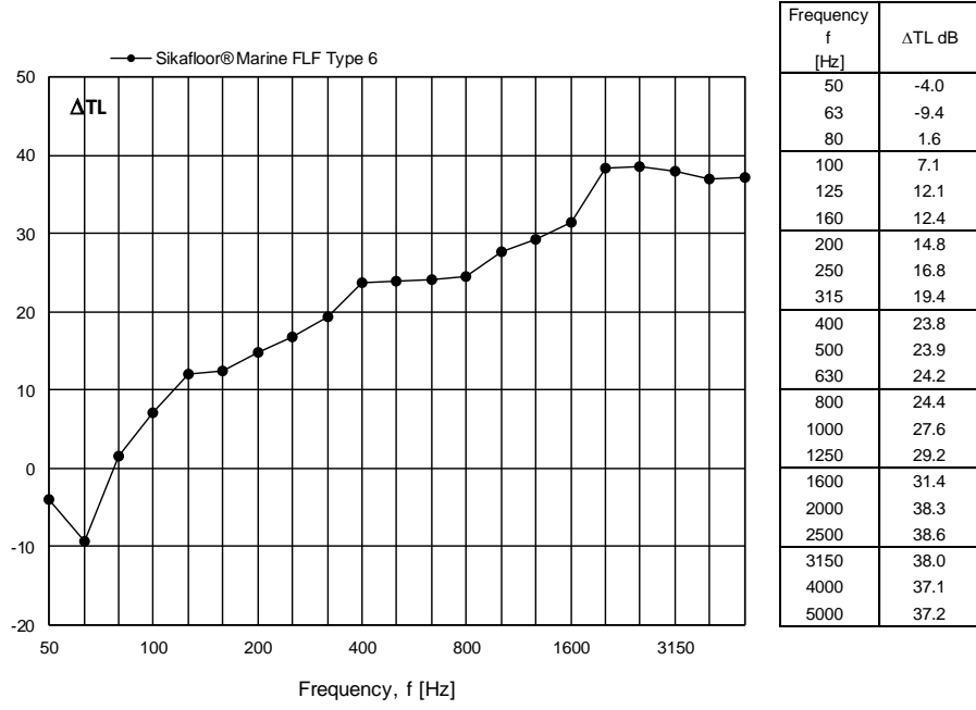
Figure 13 Measured changes in transmission loss TL for Sikafloor® Marine FLF Type 6 expressed in dB per one-third octave frequency band.
