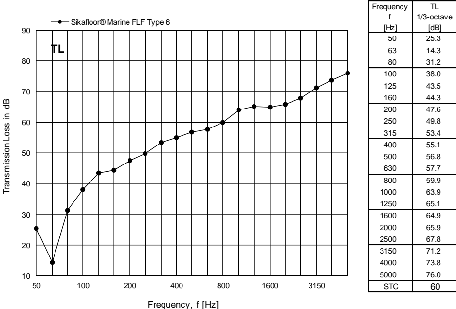
Figure 10 Measured transmission loss TL for Sikafloor® Marine FLF Type 6 expressed in dB per one-third octave frequency band.
