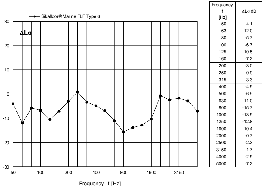
Figure 15 Measured change in radiation efficiency for Sikafloor® Marine FLF Type 6 expressed in dB per one-third octave frequency band.
