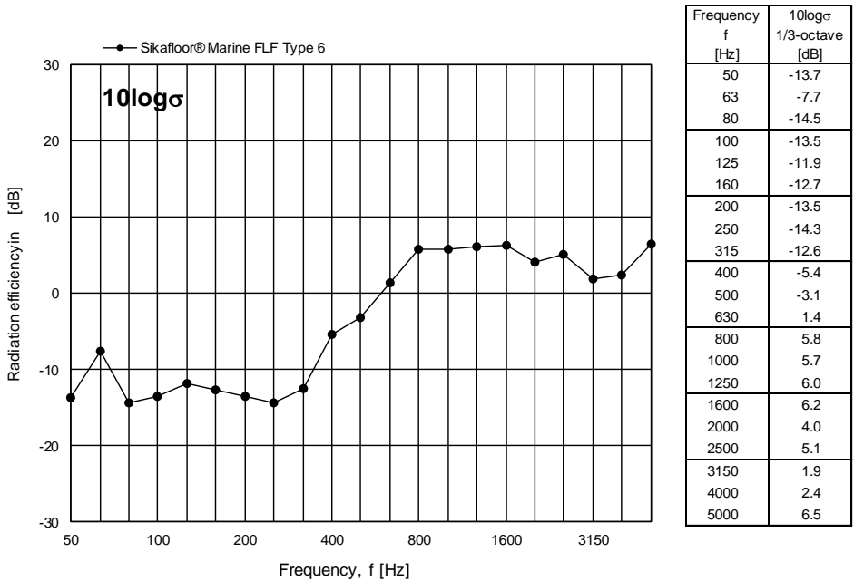
Figure 9 Measured radiation index 10 \log \sigma for Sikafloor® Marine FLF Type 6 expressed in dB per one-third octave frequency band.
