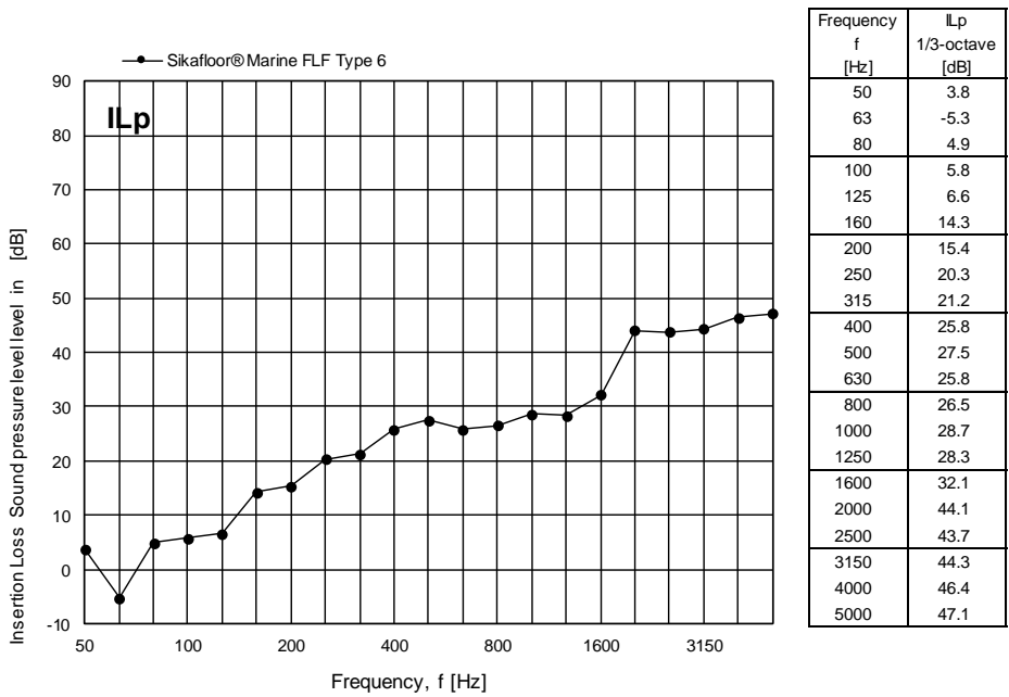
Figure 8 Measured insertion loss IL_p for Sikafloor® Marine FLF Type 6 expressed in dB per one-third octave frequency band. The insertion loss IL_p refers to the radiated mean sound pressure level in dB re 20 \mu Pa in the receiving room above the floor.
