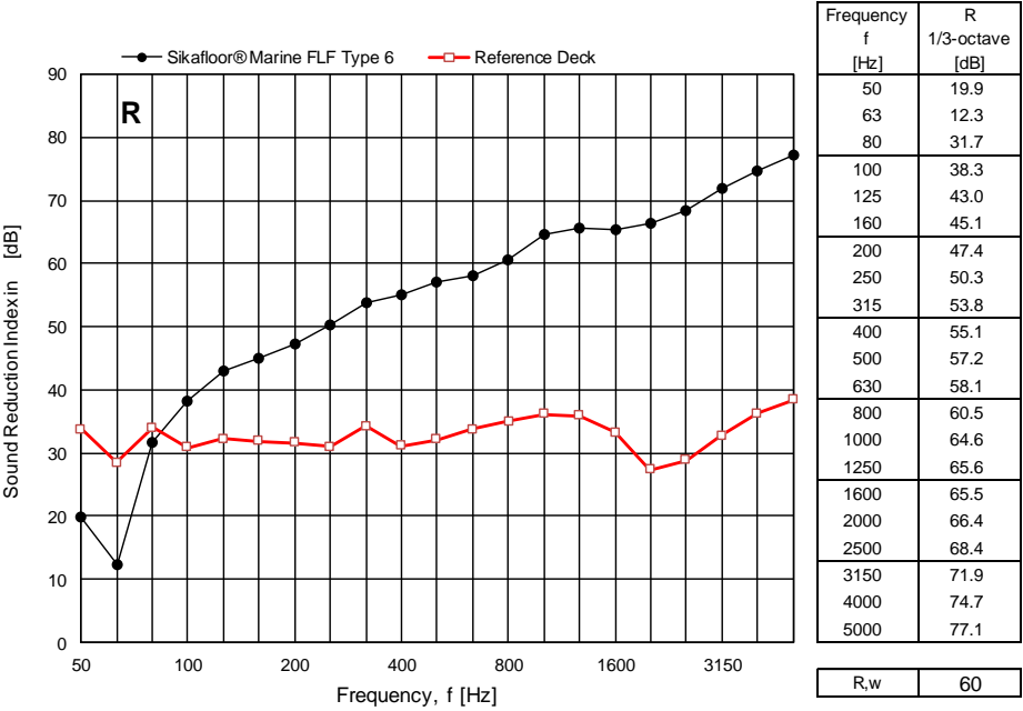
Figure 4 Measured sound reduction index R for the SikaFloor® Marine FLF Type 6 expressed in dB per one-third octave frequency bands. For comparison the results of the measurements on the bare steel deck are also shown.
